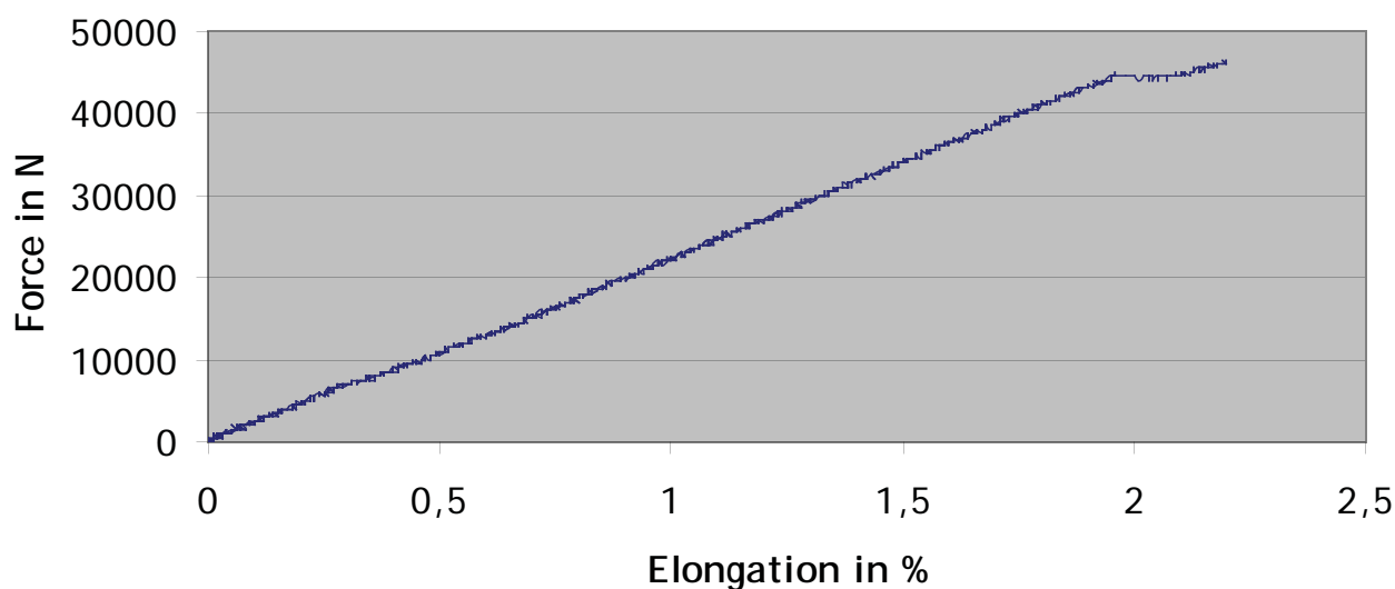
Force/Elongation ABC tape
